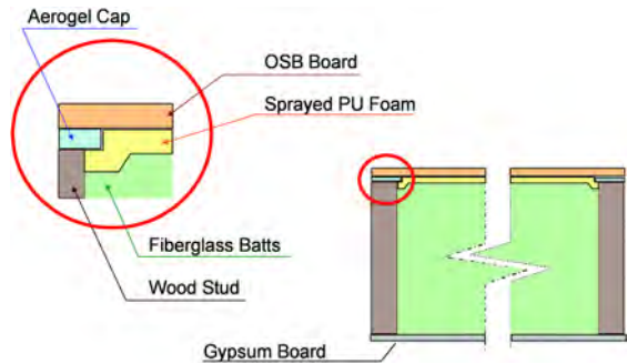
Figure 2 Wall configuration for the hot-box test with aerogel caps.
