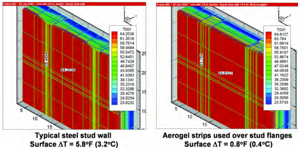
Figure 4 Simulated temperature fields on the interior-wall surfaces in two configurations of steel-frame walls.
