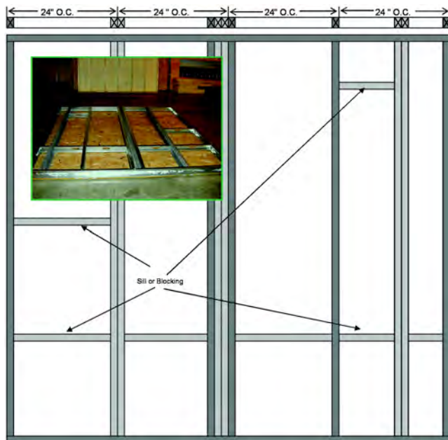
Figure 3 Configuration of the test steel stud walls.
