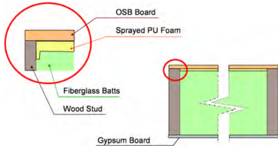
Figure 1 Material configuration for the hot-box test of the wall using fiberglass and foam cavity insulation.
